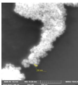
Fig. 1. SEM image of the prepared \text{Ag}_2\text{S} nanoparticles.
